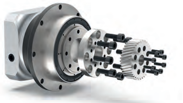
PSFNpro090 with adapter flange (064 → 090) and PM1 pinion for gearbox frame size 064
