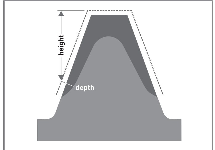
Tooth-by-tooth induction hardening
